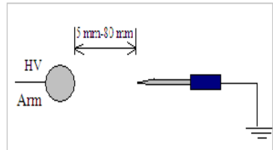
Fig 8 SPHERE-POINT arrangement
