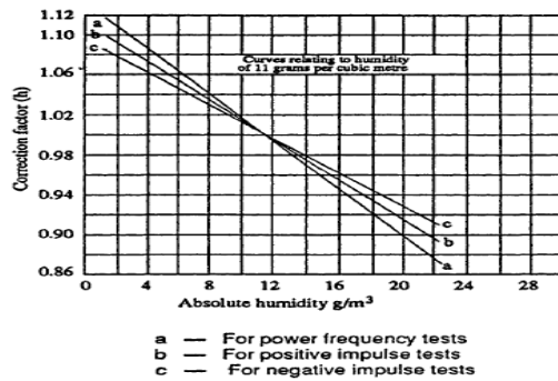
Fig. 3 Humidity correction factor
