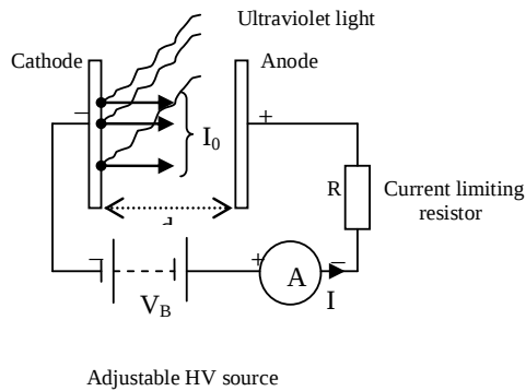
Fig 1 Test arrangement for Townsend's Discharge
