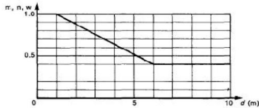
Fig. 4. Values of the Exponents m and n for Air Density Correction and w for Humidity Corrections, as a Function of Spark over Distance, in Meters.
