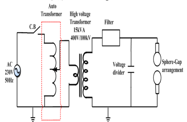
Fig 6 Schematic Circuit showing the source and Breakdown voltage measuring unit using standard sphere gap method.
