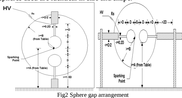
Fig2 Sphere gap arrangement
